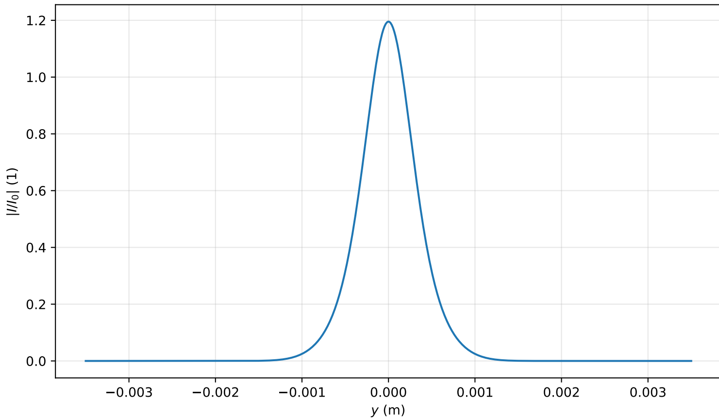
Intensity profile I(x=0, y, z=0.955)/I_0 , P_{in}=0.7P_{cr} , artificial time
